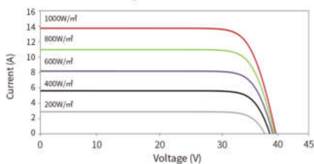
Current-Voltage Curves
