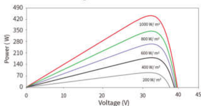
Power-Voltage Curves
